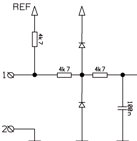
Figure 26, Input circuit (channel 1)
