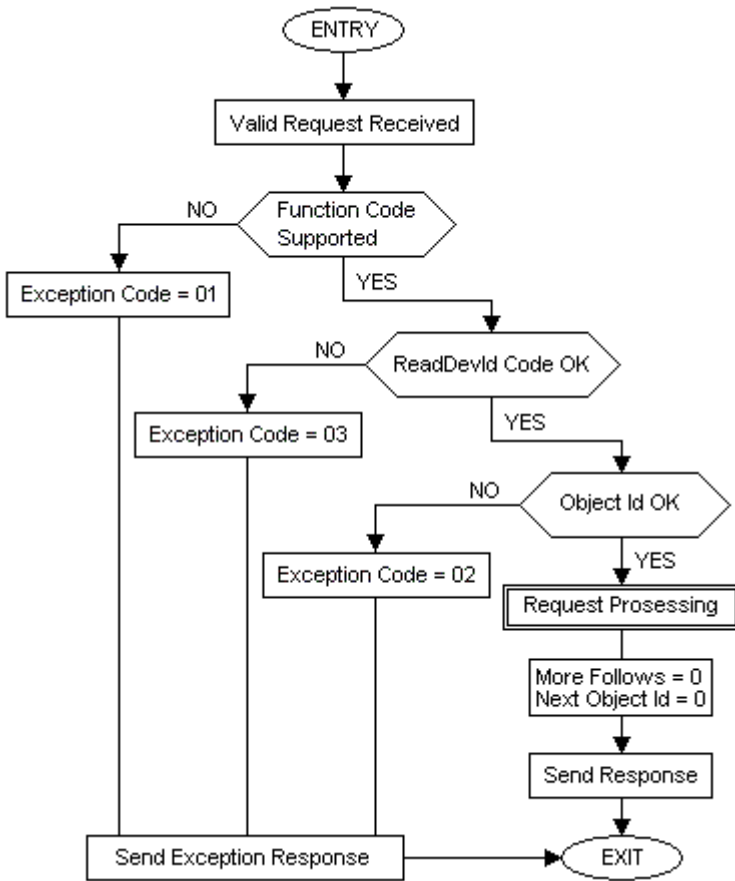
Figure 11, Read Device Identification state diagram
