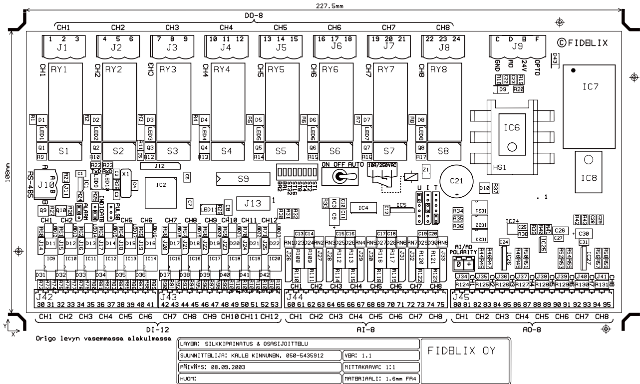
Figure 28, 36-Channel Combi Module, component placement
