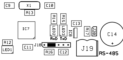
Figure 3, Short-circuiting pins 2 and 3 to enter firmware version check (AO-8 module)
