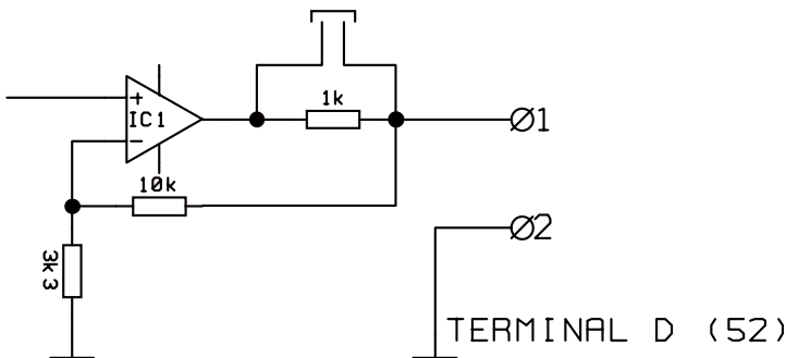
Figure 22, Analog output circuit (Channel 1)
