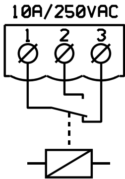
Figure 16, Output circuit (Channel 1)
