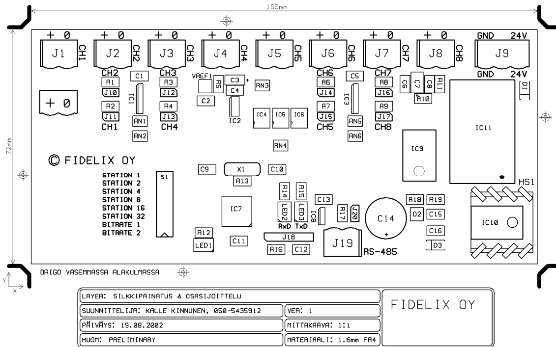
Figure 21, 8-Channel Analog Output Module, component placement
